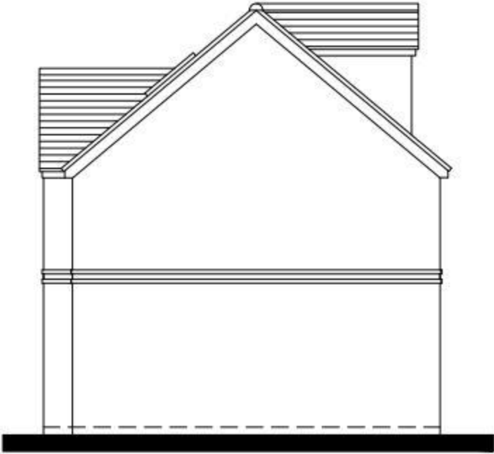
SOUTH EAST ELEVATION 1-100
